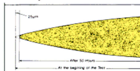
Test of Wear with the PD Needle
