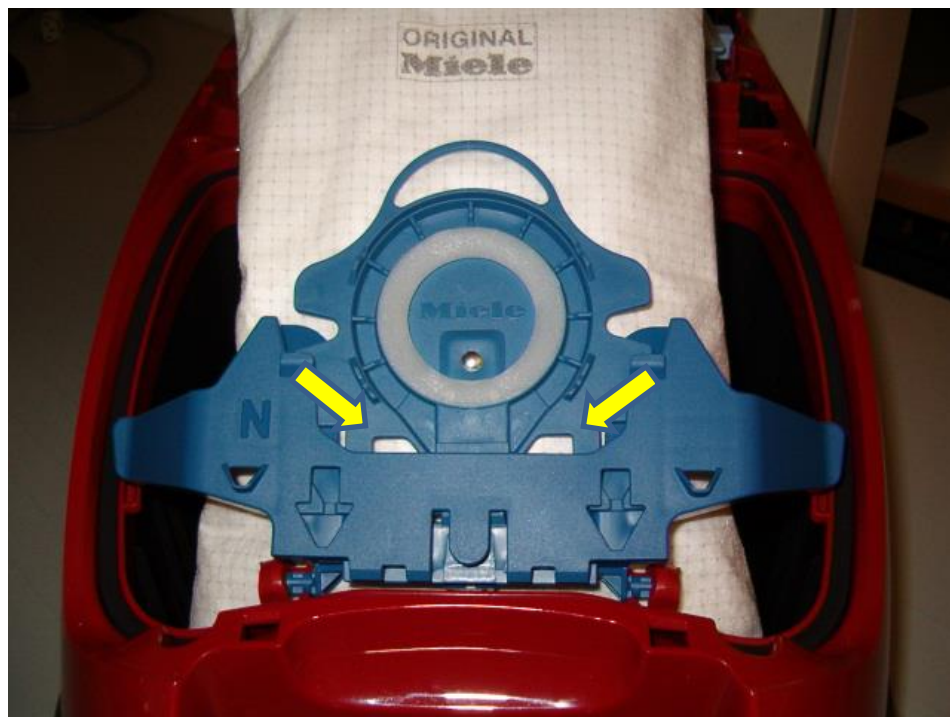
Dust bag NOT properly installed – bag is just slightly out of the holder
